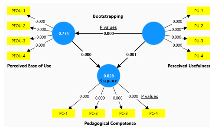
Figure 3. Bootstrapping output
